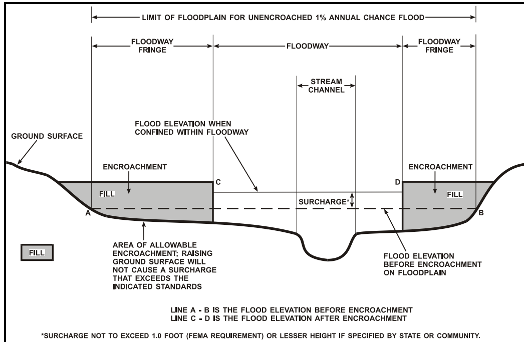
Figure 1 – Floodway Schematic
