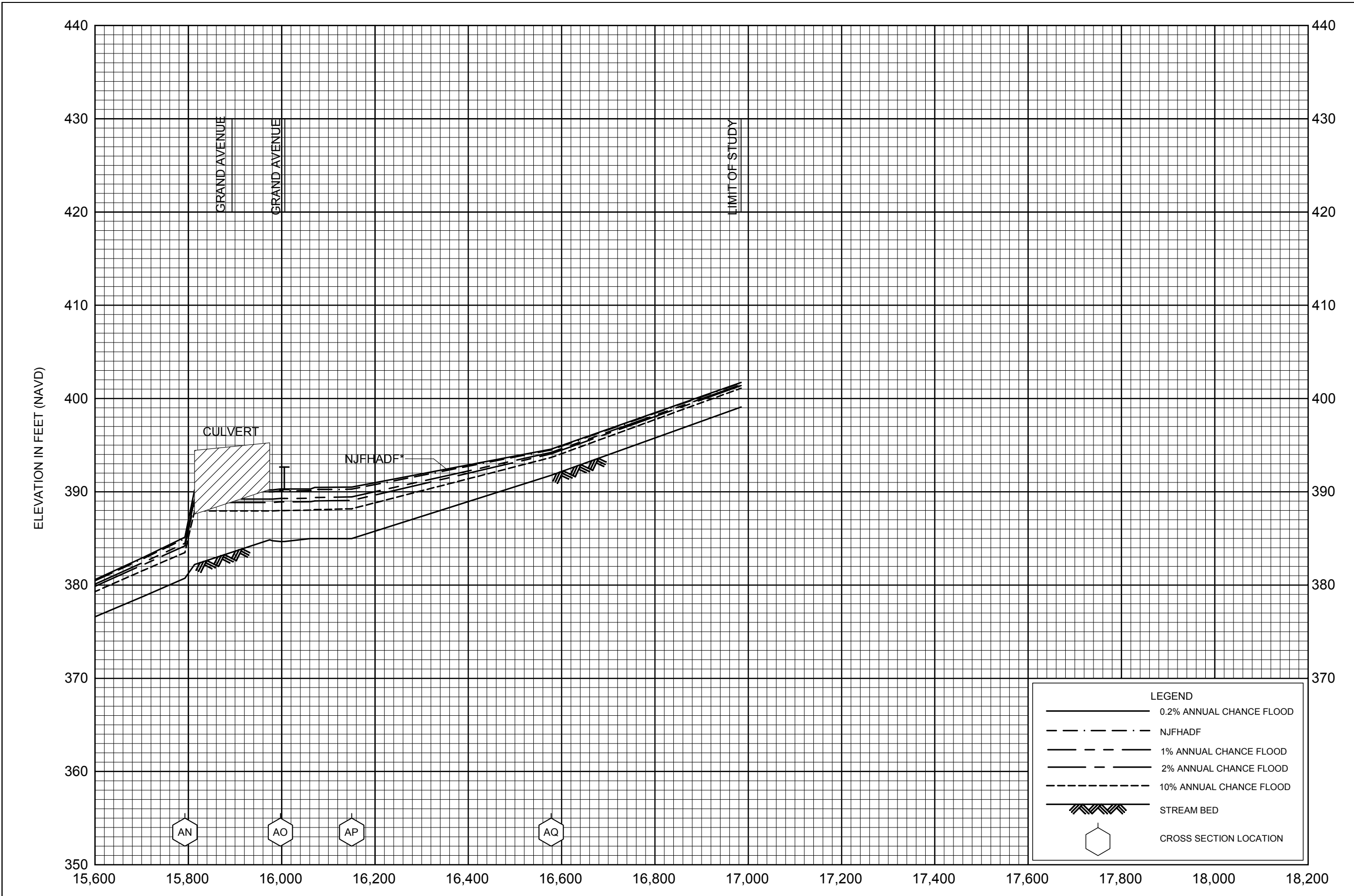
STREAM DISTANCE IN FEET ABOVE CONFLUENCE WITH PASCACK BROOK
