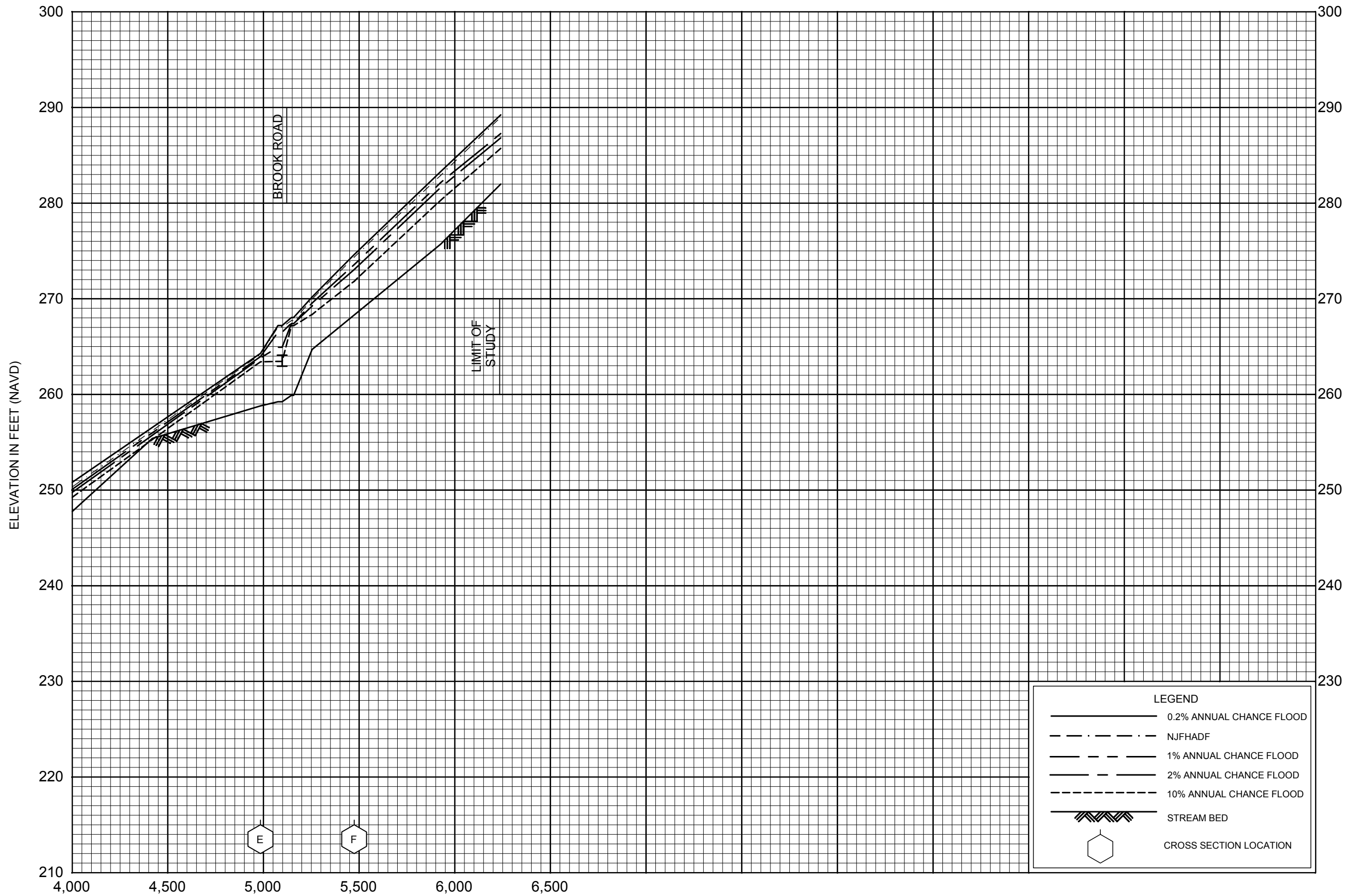
STREAM DISTANCE IN FEET ABOVE CONFLUENCE WITH SADDLE RIVER
