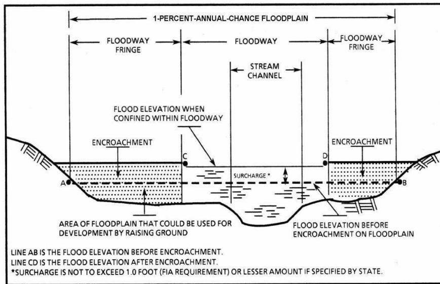
FIGURE 2: FLOODWAY SCHEMATIC
