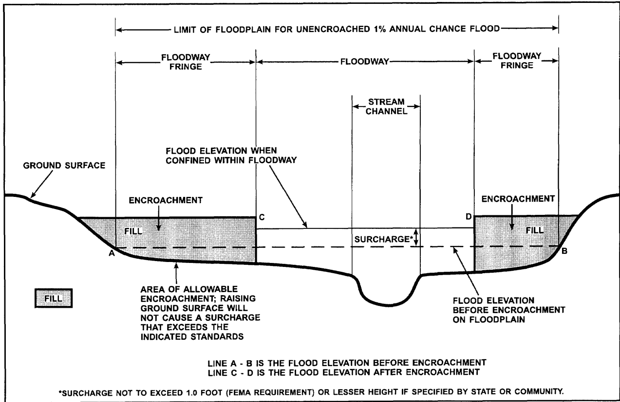
FLOODWAY SCHEMATIC
